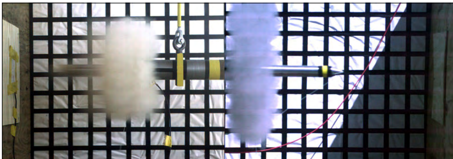
A typical composite high-speed video photograph showing the projectile ( left ) and reaction mass ( right ) just after they exited the Davis gun tube. The black powder gases appear to be of different colors because of differences in the available lighting. The real-time video showed that the Davis gun exhibited little to no pendulum motion during the five test shots, indicating that the momentums of the projectile and reaction mass were balanced.
