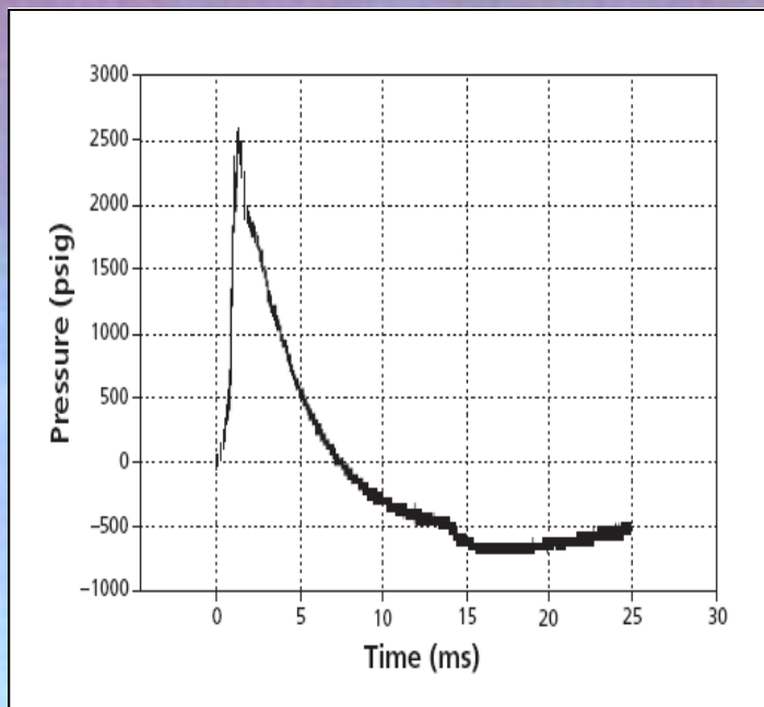
Measured Davis gun chamber pressure for a shot in which one tube of the charge bank was fired to provide a baseline for multiple-tube shots. Of particular interest here is the pressure rise time because it is one of the variables we want to tailor to simulate an acceleration square wave.
