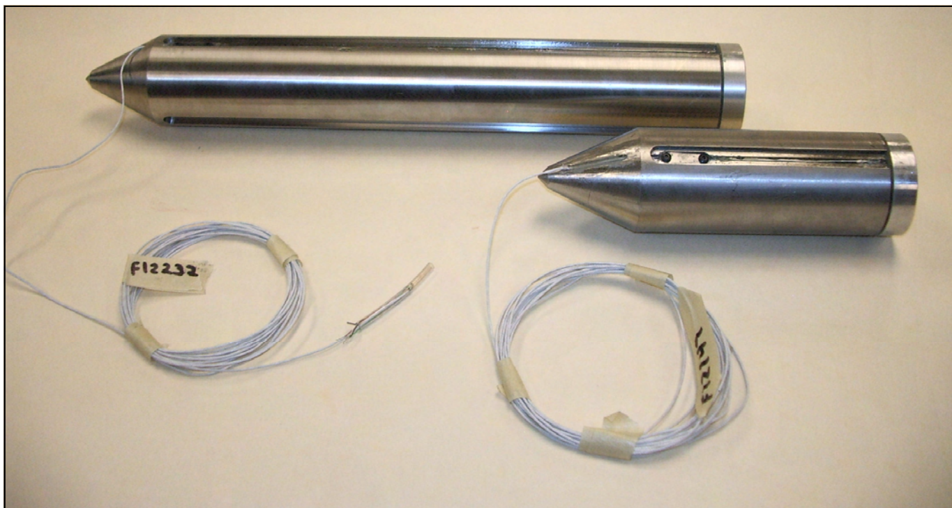
The reaction mass (top) and projectile (bottom) fired from the Davis gun, with accelerometer wires attached to their nose cones. The reaction mass weighed 12.3 lb, and the projectile weighed 3.9 lb. Each had three lengthwise grooves for phenolic resin runners that provided support in the gun barrel and reduced friction. Plastic disks (not shown) at the base ends of the reaction mass and projectile acted as pressure seals.
