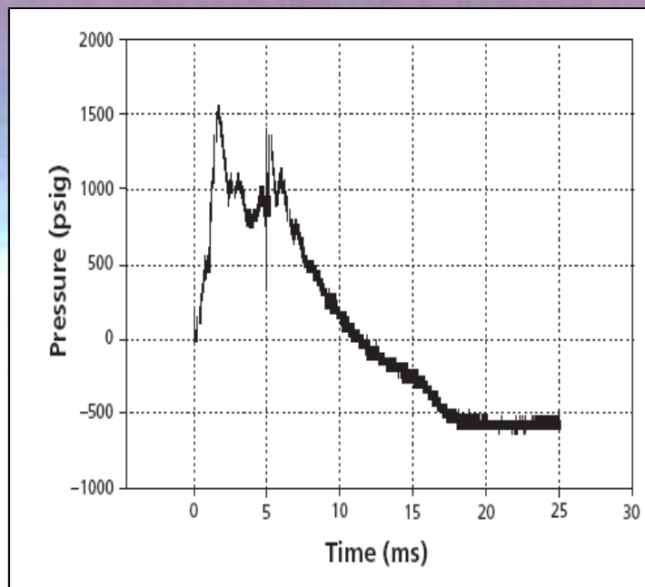
Measured Davis gun chamber pressure for a shot in which two tubes of the charge bank were fired with a 5.0-ms delay. Fast-burning black powder is fired in two or more tubes to achieve both a rapid rise time and pressures that remain high for up to 10 ms. The goal of tailoring the pressure pulse is to produce an acceleration pulse that approximates a square wave such as occurs during projectile earth-penetration deceleration.
